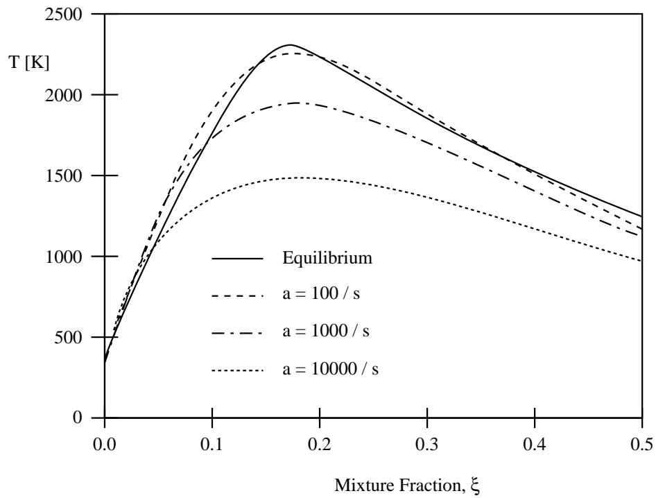
Fig. 12.3: Temperature profiles from flamelet calculations at different strain rates.
