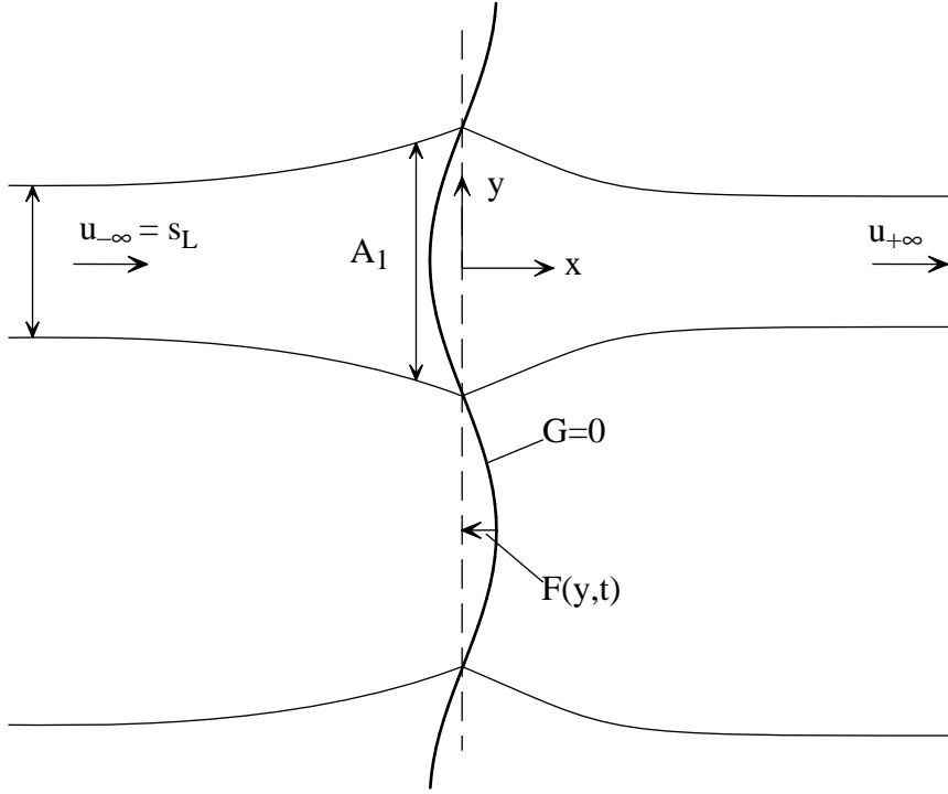
Fig. 8.5: Illustration of the hydro-dynamic instability
